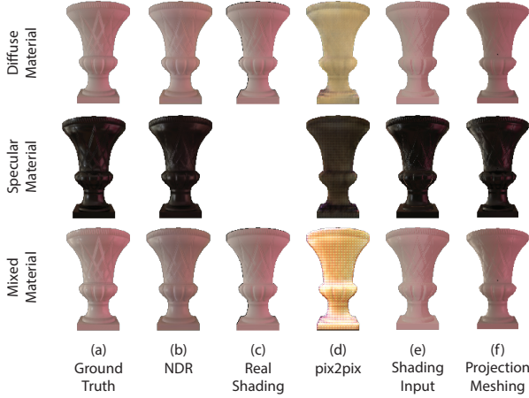
Figure 6: Comparison of images rendered by the NDR and comparable methods under fixed illumination. The same object is shown with a material that is purely diffuse, purely specular, and a mixture of both. The model "Decorative Vase" by fresherator2 [fre20] is licensed under CC BY 4.0 [Crea].
