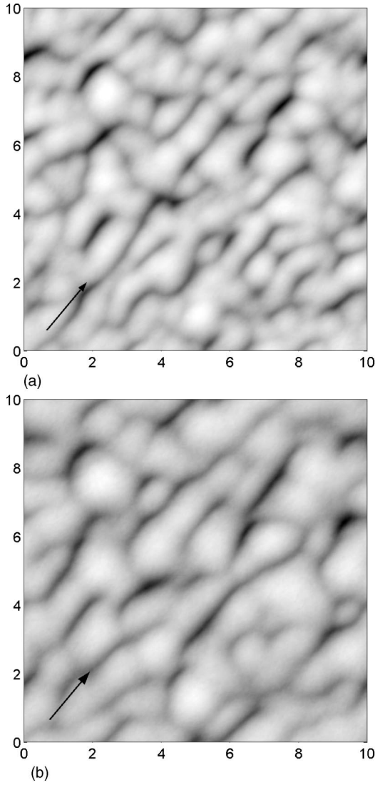
FIG. 4. 10 \times 10 \mu\text{m}^2 simulations generated using the MBE equation with growth times of (a) 10 min and (b) 37.5 min. The scale bars are in nm, and the arrows point along the [\bar{1}10] direction. The fourth order equation also produces a mounded surface, although the depth of the cusps between the mounds is greater than on the real surfaces.
