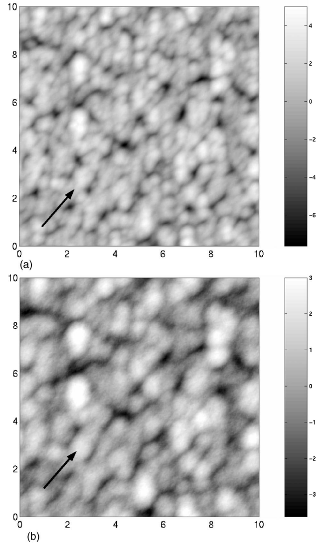
FIG. 3. 10 \times 10 \mu\text{m}^2 simulations generated using the conservative form of the KPZ equation with growth times of (a) 10 min and (b) 37.5 min. The scale bars are in nm, and the arrows point along the [1\bar{1}0] direction. The simulations compare well with the real surfaces shown in Fig. 2.
