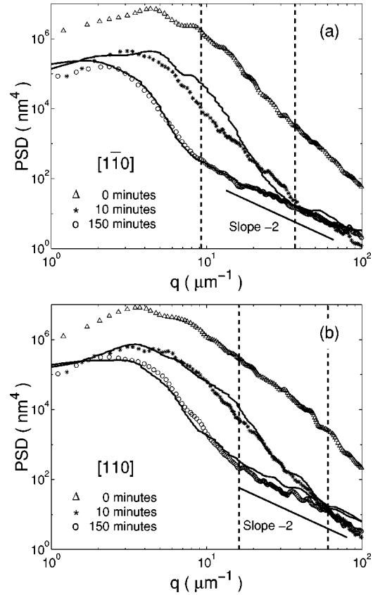
FIG. 5. PSD after different growth times on thermally cleaned substrates, measured along (a) the [\bar{1}10] direction and (b) the [110] direction. The symbols represent the experimental data. The solid lines, representing 10 and 150 min simulations generated with the KPZ equation, are in excellent agreement with the experimental data. The vertical dashed lines indicate the cutoff frequencies q_c at 10 and 150 min (right to left).
