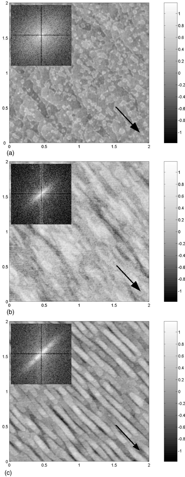
FIG. 12. 2 \times 2 \mu\text{m}^2 AFM images illustrating the effect of reducing the \text{As}_2 overpressure. (a) V:III ratio=6.5 (sample H3), (b) V:III ratio=3.0 (sample H4), and (c) V:III ratio=1.0 (sample H5). The scale bars are in nm, and the surface features are elongated along the [1\bar{1}0] direction (along the arrow). The 2D PSD of each image is included as an inset, with spatial frequencies ranging from -300 to 300 \mu\text{m}^{-1} in each direction.
